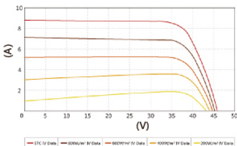
I-V Curve ( JY365M6-Ga-5 )
